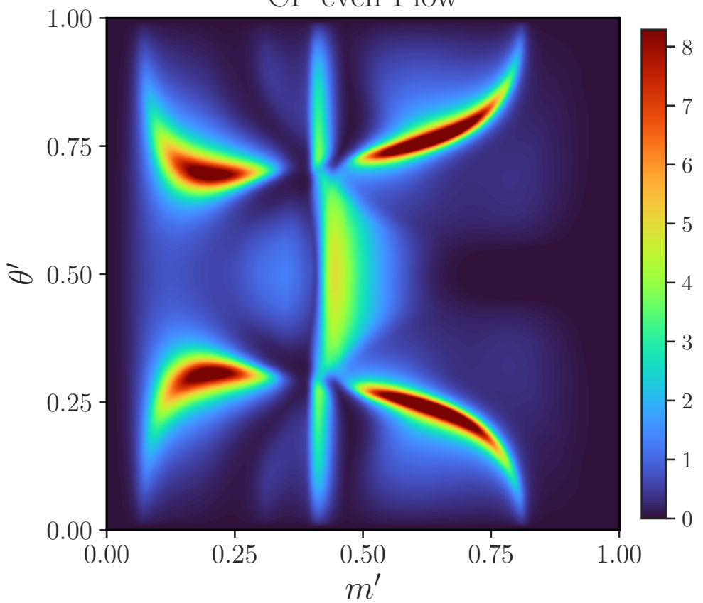
CP-even Flow
