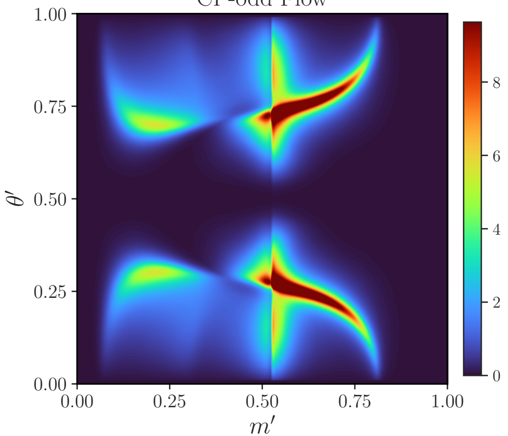
CP-odd Flow
